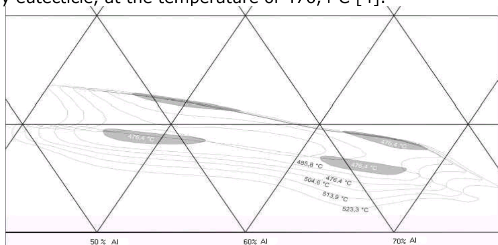
Fig.4 The projection on the Gibbs triangle of the isotherms form the zone of the ternary eutectic. The area delimited by the isotherm of 476,4°C.
