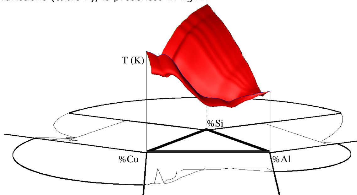
Fig. 1 The computerised generation of the liquidus surface from the ternary diagram Al-Cu-Si
