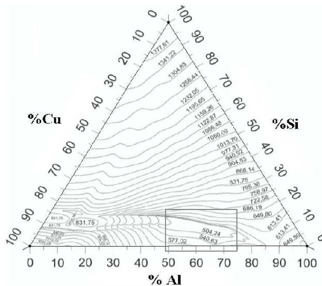
Fig.3 The projection of the liquidus surface on the plane of the Gibbs triangle and the delimitation of the ternary eutectic area.
