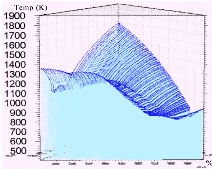
Fig.2 The liquidus surface mathematically modelled, in the ternary system Al-Cu-Si.
