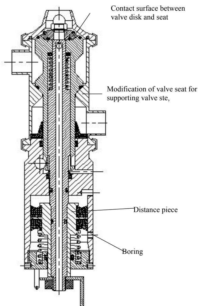
FIGURE 4. THE CUTAWAY VIEW OF THE MODIFIED VALVE
