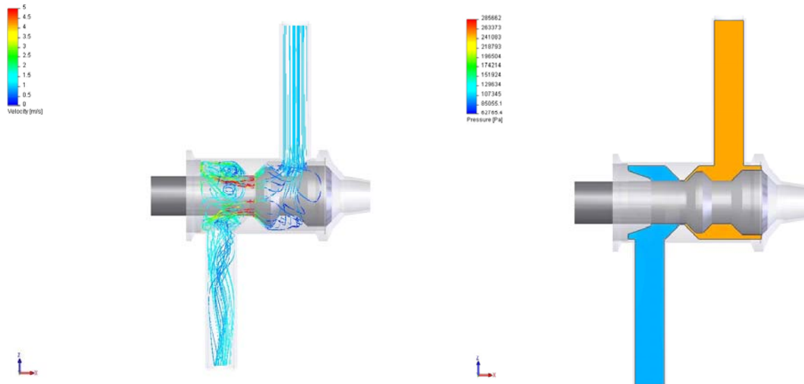
FIGURE 2. CHANGING OF THE FLOW VELOCITY AND PRESSURE IN THE VALVE
