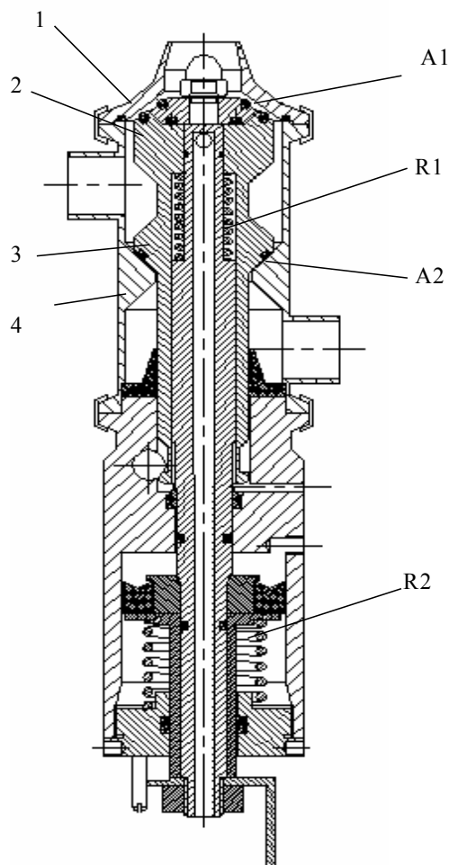
FIGURE 1. THE CUTAWAY VIEW OF VALVE
