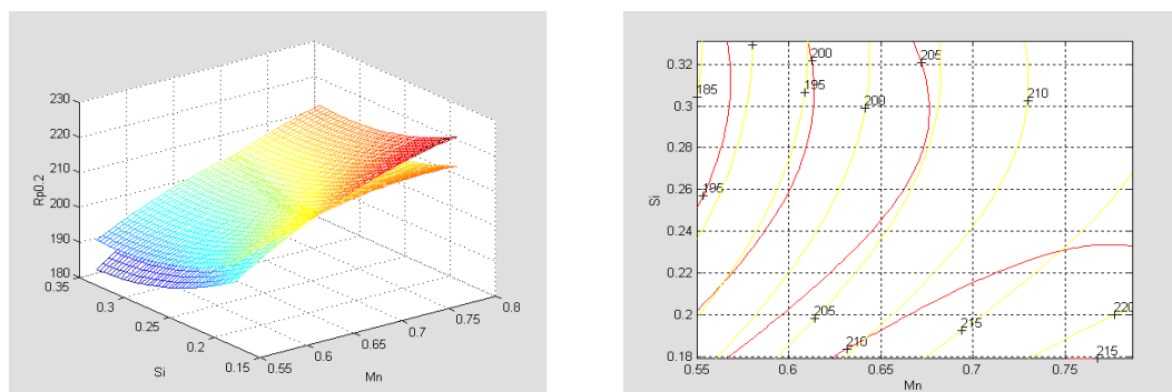
FIG.5 THE DELIMITATION OF THE BEST FIELD FOR THE TECHNICAL RUNNING LIMIT R_{P0,2/450} , DEPENDING ON THE MANGANESE AND SILICIUM CONTENT, TAKING INTO CONSIDERATION THE MEDIUM PERCENTAGE OF CARBON
