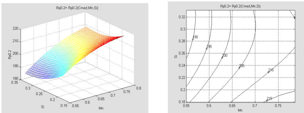
FIG.2. THE VARIATION OF THE TECHNICAL RUNNING LIMIT R_{p0,2/450} , CONTAINING MANGANESE AND SILICIUM, TAKING INTO CONSIDERATION THE MEDIUM PERCENTAGE OF CARBON
