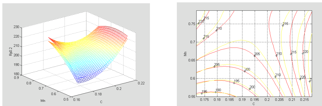
FIG.7 THE DELIMITATION OF THE BEST FIELD FOR THE TECHNICAL RUNNING LIMIT R_{P0,2/450} , DEPENDING ON THE CARBON AND MANGANESE CONTENT, TAKING INTO CONSIDERATION THE MEDIUM PERCENTAGE OF SILICIUM
