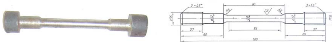
FIG.1 THE SHAPE AND SIZE OF TEST-BARS USED IN TESTING
