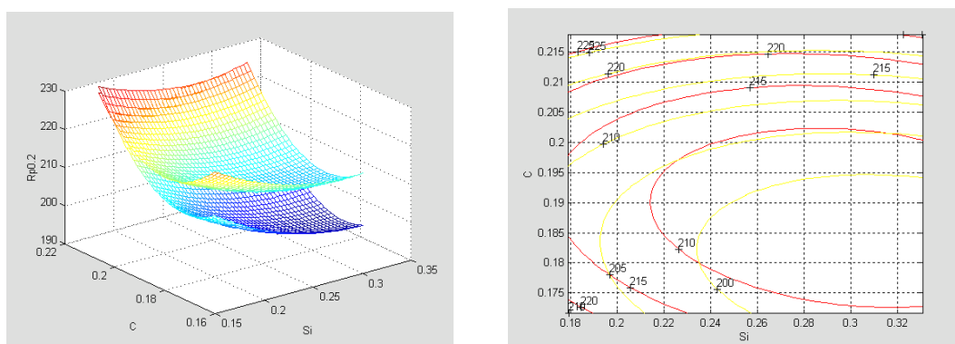
FIG.6 THE DELIMITATION OF THE BEST FIELD FOR THE TECHNICAL RUNNING LIMIT R_{P0,2/450} , DEPENDING ON THE CARBON AND SILICIUM CONTENT, TAKING INTO CONSIDERATION THE MEDIUM PERCENTAGE OF MANGANESE
