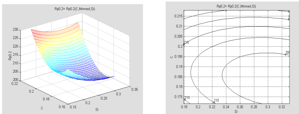
FIG.3 THE VARIATION OF THE TECHNICAL RUNNING LIMIT R_{p0,2/450} , CONTAINING CARBON AND SILICIUM, TAKING INTO CONSIDERATION THE MEDIUM PERCENTAGE OF MANGANESE
