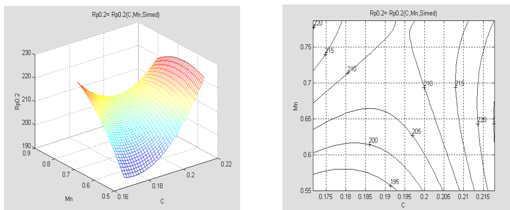
FIG.4 THE VARIATION OF THE TECHNICAL RUNNING LIMIT R_{p0,2/450} , CONTAINING MANGANESE AND CARBON, TAKING INTO CONSIDERATION THE MEDIUM PERCENTAGE OF SILICIUM
