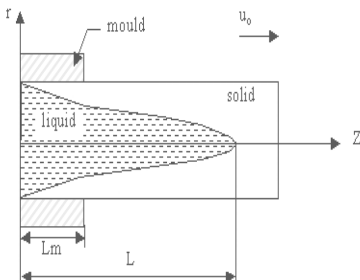
FIGURE 3: R-Z COORDINATES ATTACHED TO MOULD
