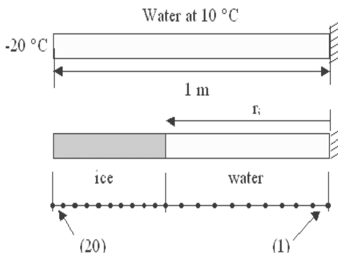
FIGURE 4. MODELING OF THE ONE DIMENSIONAL PROBLEM
