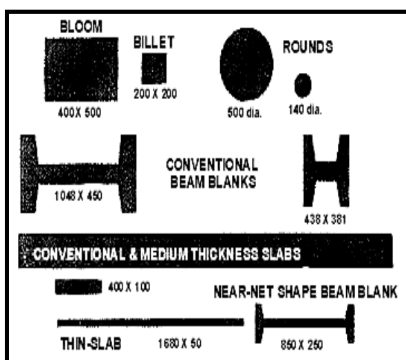
FIGURE 2: CONTINUOUSLY CAST SECTIONS
