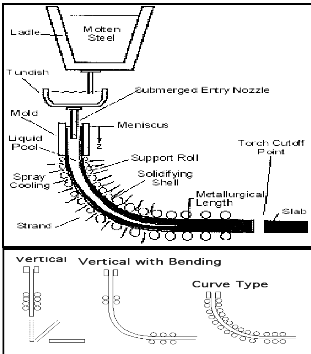
FIGURE 1. SCHEMATIC REPRESENTATION OF THE CONTINUOUS CASTING PROCESS
