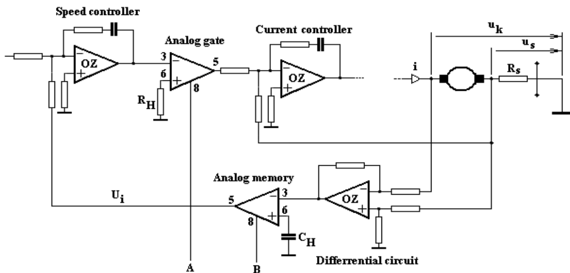
Figure 3. The speed control system circuit without tachogenerator
