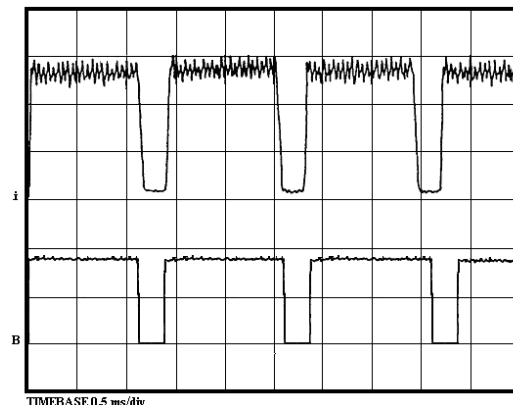
Figure 7. The analog gate control signal and the current signal
