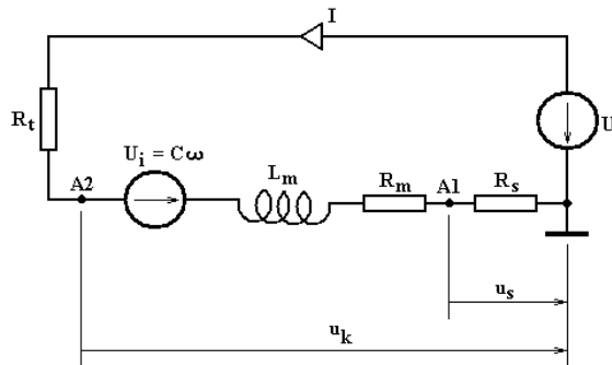
Figure 2. The Motor Armature Circuit In Normal Operating Mode
