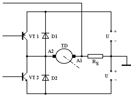
Figure 1. The Motor Armature Circuit
