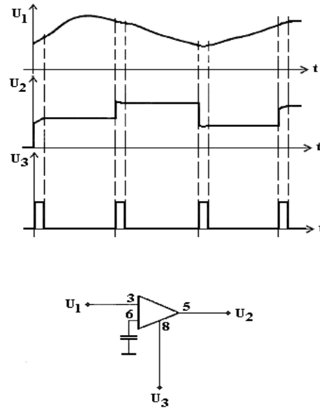
Figure 5. The operation of an analog memory
