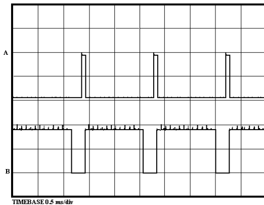
Figure 6. The analog gate and memory control signals
