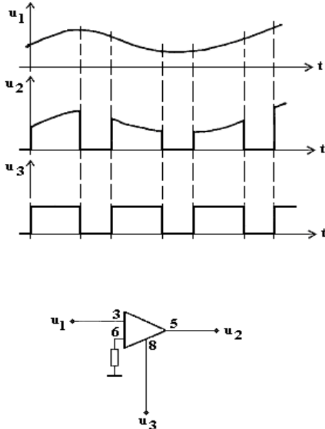
Figure 4. The operation of an analog gate
