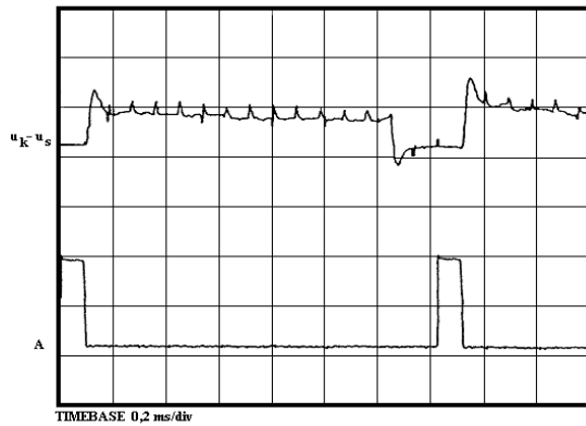
Figure 8. The voltage at the motor terminals and the analog memory control signal
