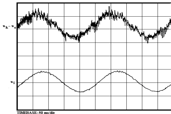
Figure 10. The voltage at the motor terminals and the output voltage of the analog memory
