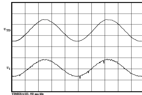
Figure 11. The comparison of tg voltage and the voltage at the output of analog memory
