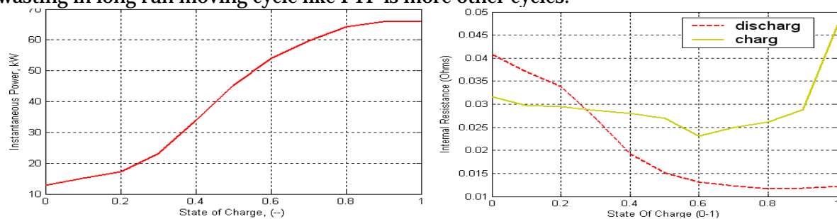
Figure 7. Variation of internal resistance and power of a battery versus charging states [16]
