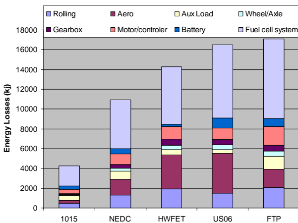
Figure6. Energy wasting in various part of a vehicle for different moving cycle
