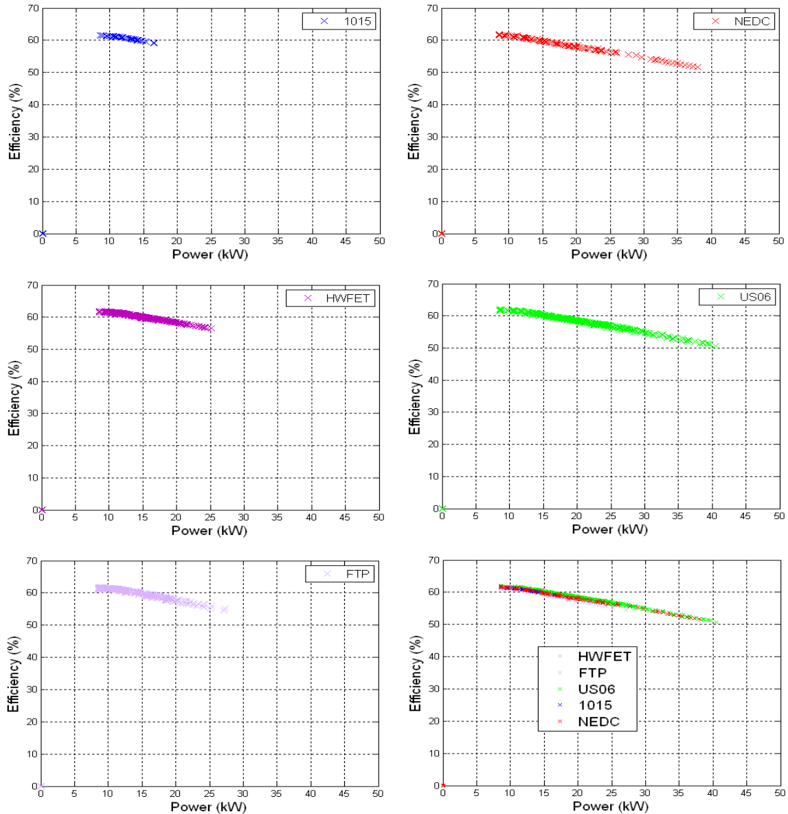
Figure8. Efficiency versus power in different moving cycle
