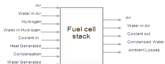
Figure 3. Block diagram simulation of fuel cell
