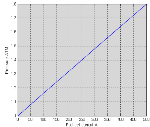
Figure 2. Strategy control of operating pressure
