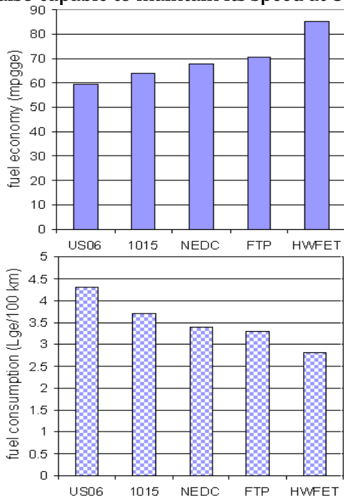
Figure 5: comparing the fuel consumption and economy in different moving cycle
