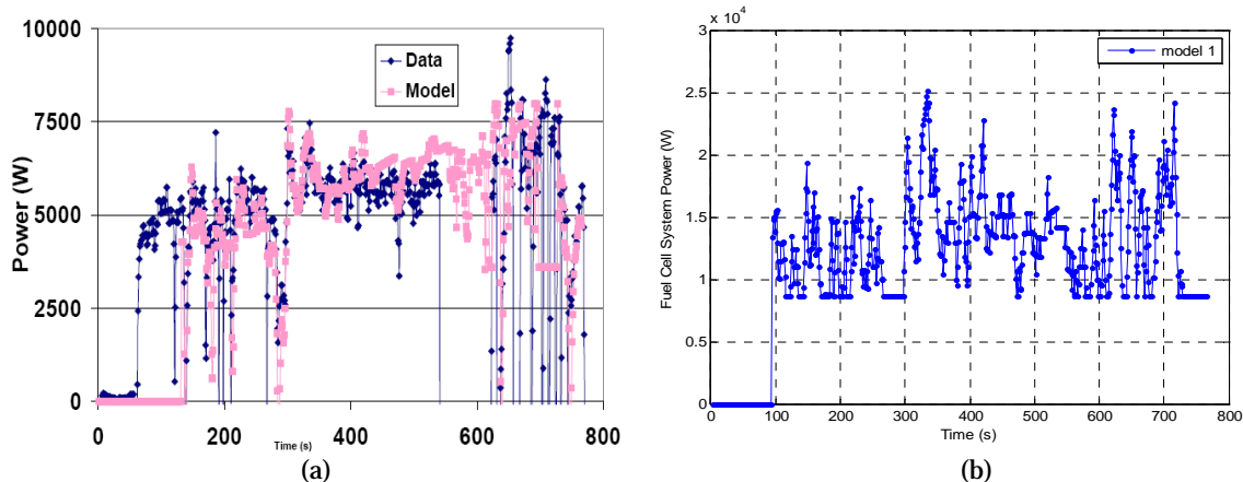
Figure 4- comparing power system variation of the fuel cell versus time regarding moving cycle HWFET, in the reference 14 figure (a) and the present paper figure (b)
