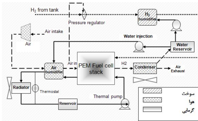
Figure 1. Fuel cell system in vehicle
