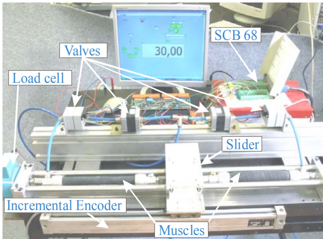
Figure 2. The photo of the experimental setup
