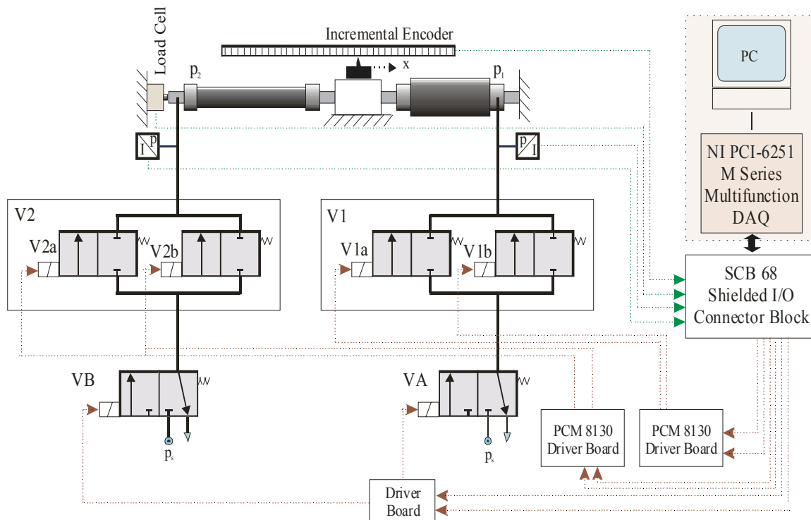
Figure 3. Configuration of pneumatic positioning system
