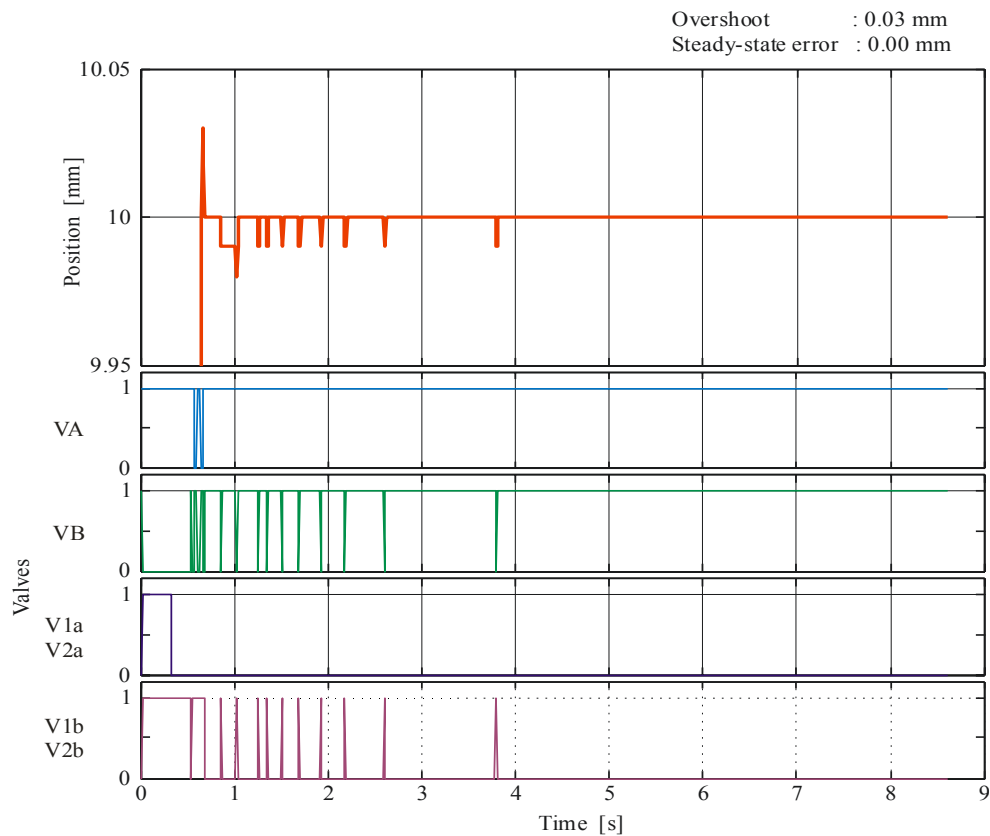
Figure 7. The time functions of the position and control signal (enlarged)
