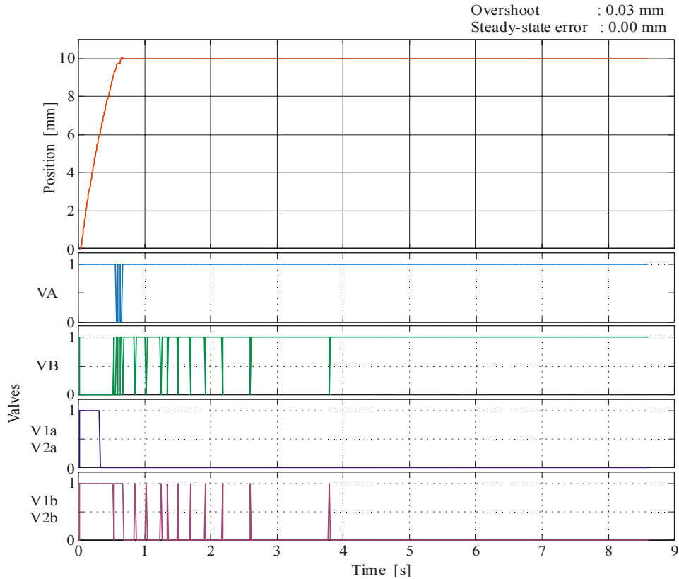
Figure 6. The time functions of the position and control signal
