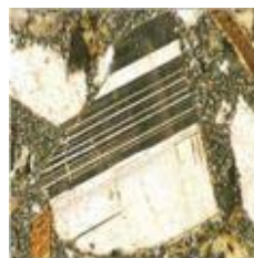
c, Na-Ca feldspar in andesite 50x
