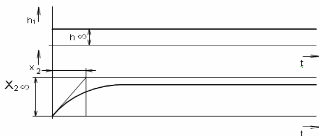
Figure 3. Transient curve of process as a controlled system S referring to its transition s_{x_2}
