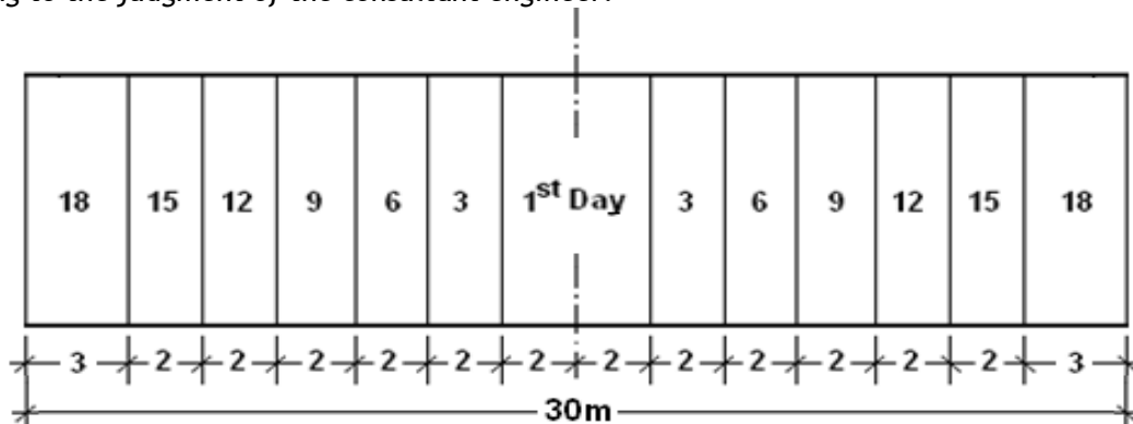
Figure 7. Suggested Concrete Casting Sequence for a Bridge Deck Slab Spanning 30m
