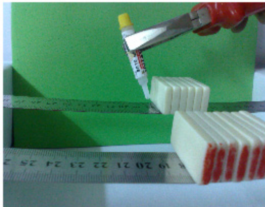
Figure 3. Gluing Plastic Prisms to the Rear Ruler RA
