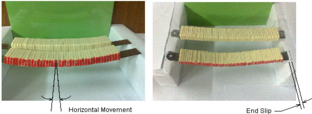
Figure 6. Horizontal Movement and End Slip in Specimen RB
