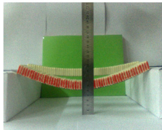
Figure 4. Deflection increase with each Loading increment Central deflections for both rulers were listed in Table1 for each additional two prisms.
