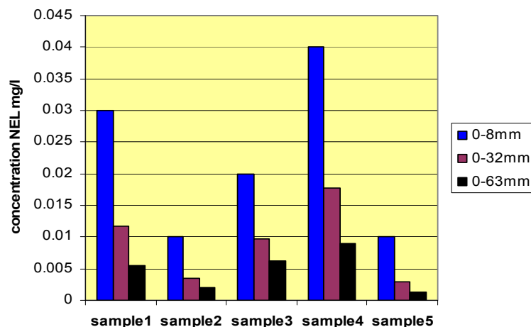
Figure 3: Effect of particle size on NEL concentration in aqueous solution (threshold limit value=0.1 mg/l). The threshold limit value of NEL concentration is 0.1 mg/l as it is evident in Figure 3, all the measured NEL concentration values are lower in all samples. Comparison of the measured Ni, Zn, Cr, Cd, Pb and Hg concentration values e.g. in sample 1 with the threshold limit values is shown in Table 4. Similar low Ni, Zn, Cr, Cd, Pb and Hg concentrations were identified in samples 2 to 5 and the effect of particle sizes on concentration of these elements in the aqueous solutions were proved.
