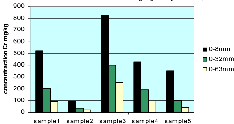
Figure 6. Effect of particle size on the Cr concentration in the dry matter (threshold limit value = 250 mg kg -1 dry matter)
