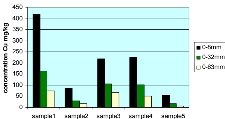
Figure 4. Effect of particle size on the copper concentration in the dry matter (threshold limit value = 100 mg kg -1 dry matter)
