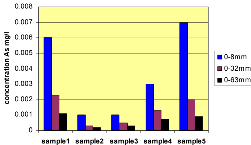
Figure 2: Effect of particle size on arsenic concentration in aqueous solution (threshold limit value=0.05 mg/l). Due to low As concentration values (see Figure 2) it can be assumed that As in rail bed samples is present in the form which is less soluble in water.
