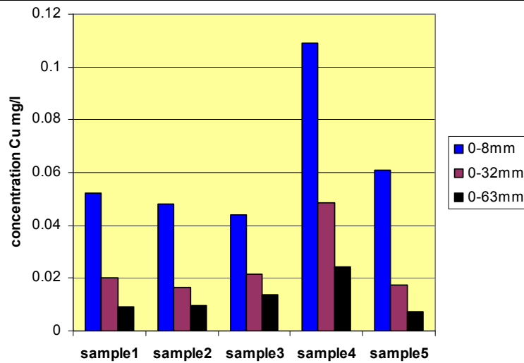
Figure 1: Effect of particle size on copper concentration in aqueous solution (threshold limit value=0.1 mg/l).
