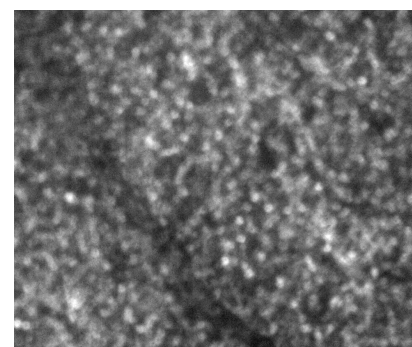
Microstructure of sample C (etched in 2% nital) X200
