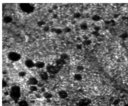
Microstructure of sample A (etched in 2% nital) X200
