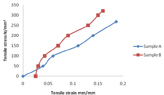
Figure 1: Stress –Strain curve for Samples A and B Stress –strain curve for sample A, Stress –strain curve for sample B
