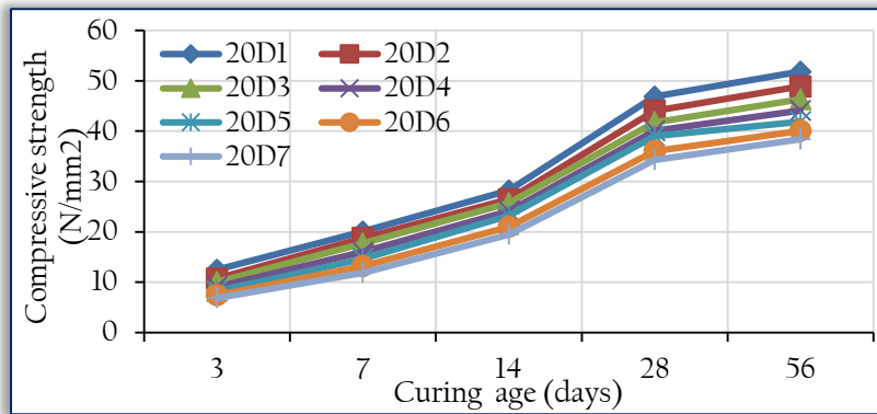
Figure 4. Relationship between the compressive strength and curing age of concrete specimens containing 20% sugar cane bagasse ash (SBA) and saw dust ash (SDA)
