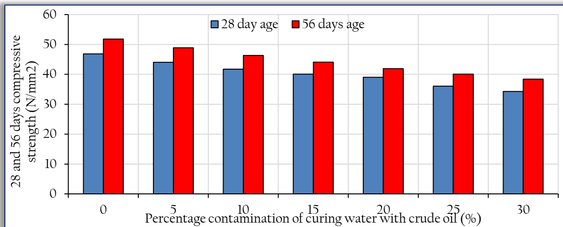
Figure 5. Relationship between the percentage contaminations of curing water with 28 and 56 days compressive strength of concrete specimens containing 20% sugar cane bagasse ash (SBA) and saw dust ash (SDA)
