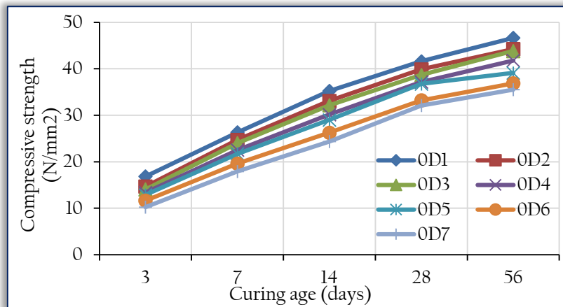
Figure 2. Relationship between the compressive strength and curing age of concrete specimens containing 0% sugar cane bagasse ash (SBA) and saw dust ash (SDA)
