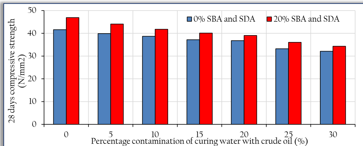
Figure 6. Relationship between the percentage contaminations of curing water with 28 days compressive strength of concrete specimens containing 0% and 20% sugar cane bagasse ash (SBA) and saw dust ash (SDA)
