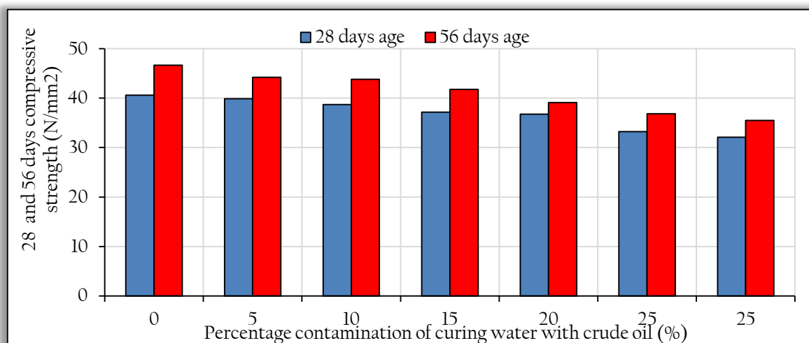
Figure 3. Relationship between the percentage contaminations of curing water with 28 and 56 days compressive strength of concrete specimens containing 0% sugar cane bagasse ash (SBA) and saw dust ash (SDA)
