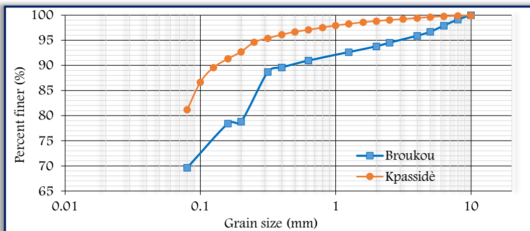
Figure 2. Particle size curves of Broukou and Kpassidè clay soils
