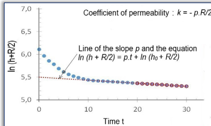
Figure 7. Permeability curve [8]
