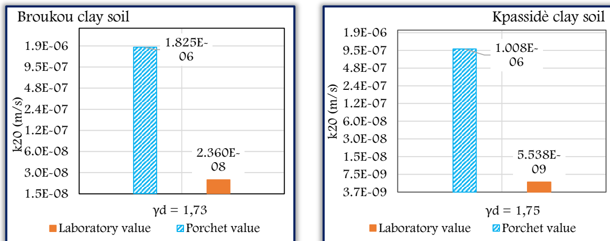
Figure 3. Comparative diagrams of Porchet and variable load permeameter tests results on Broukou and Kpassidè clays soils
