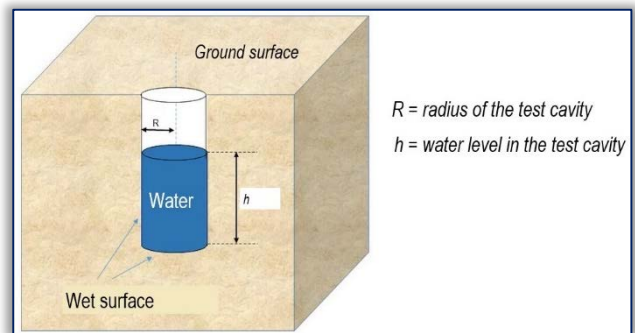
Figure 2. Principle schema of Porchet test [8]
