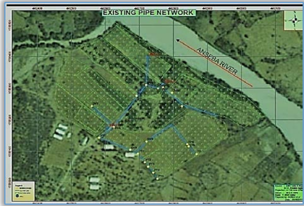
Figure 2: Existing Pipe network at HAC
