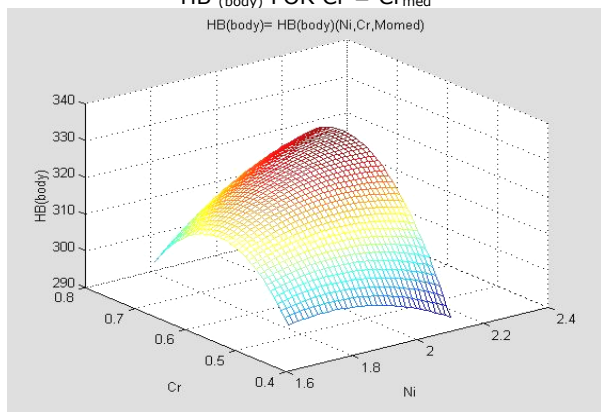
FIGURE 5. THE REGRESSION SURFACE HB (body) FOR Mo = Mo med
