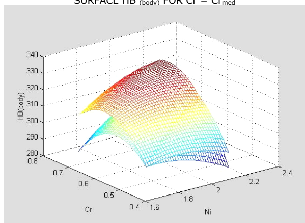
FIGURE 11. THE VOLUME VARIATION OF THE REGRESSION SURFACE HB_{(body)} FOR Mo = Mo_{med}
