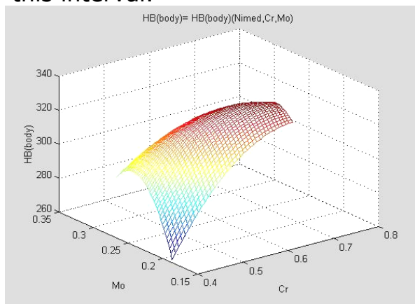
FIGURE 1. THE REGRESSION SURFACE HB (body) FOR Ni = Ni med
