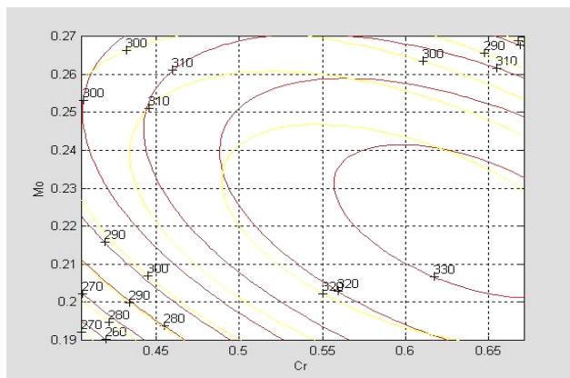
FIGURE 8. LEVEL CURVES FOR THE VOLUME VARIATION OF THE REGRESSION SURFACE HB_{(body)} FOR Ni = Ni_{med}
