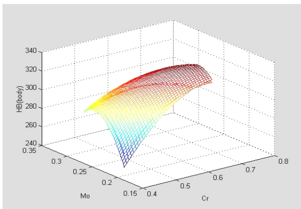
FIGURE 7. THE VOLUME VARIATION OF THE REGRESSION SURFACE HB_{(body)} FOR Ni = Ni_{med}
