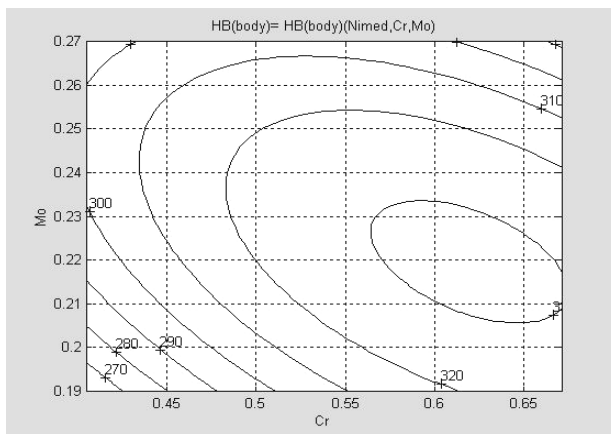
FIGURE 2. LEVEL CURVES HB (table) = f(Ni med , Cr, Mo)
