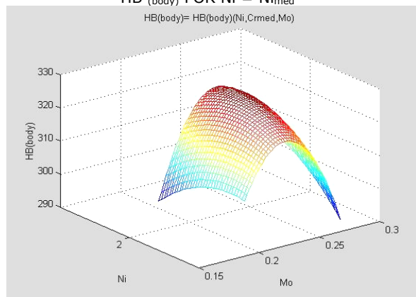
FIGURE 3. THE REGRESSION SURFACE HB (body) FOR Cr = Cr med
