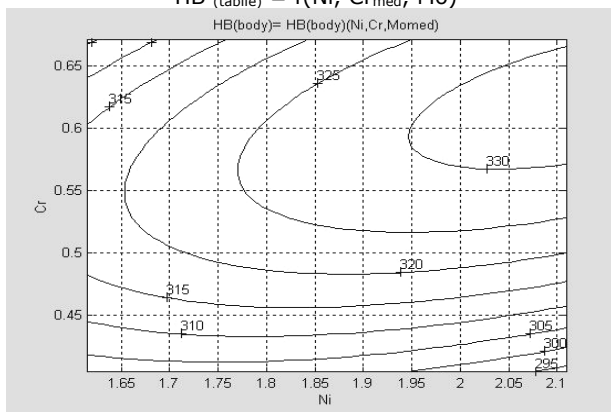
FIGURE 6. LEVEL CURVES HB (table) = f(Ni, Cr, Mo med )
