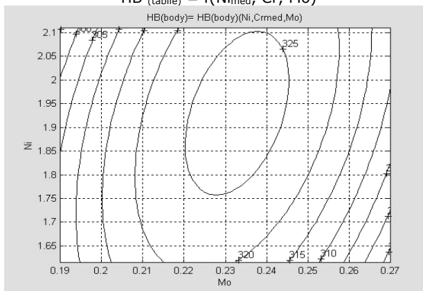
FIGURE 4. LEVEL CURVES HB (table) = f(Ni, Cr med , Mo)
