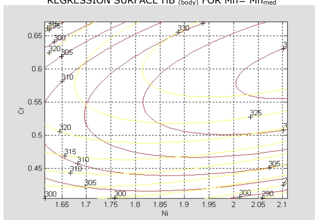
FIGURE 12. LEVEL CURVES FOR THE VOLUME VARIATION OF THE REGRESSION SURFACE HB_{(body)} FOR Mo = Mo_{med}
