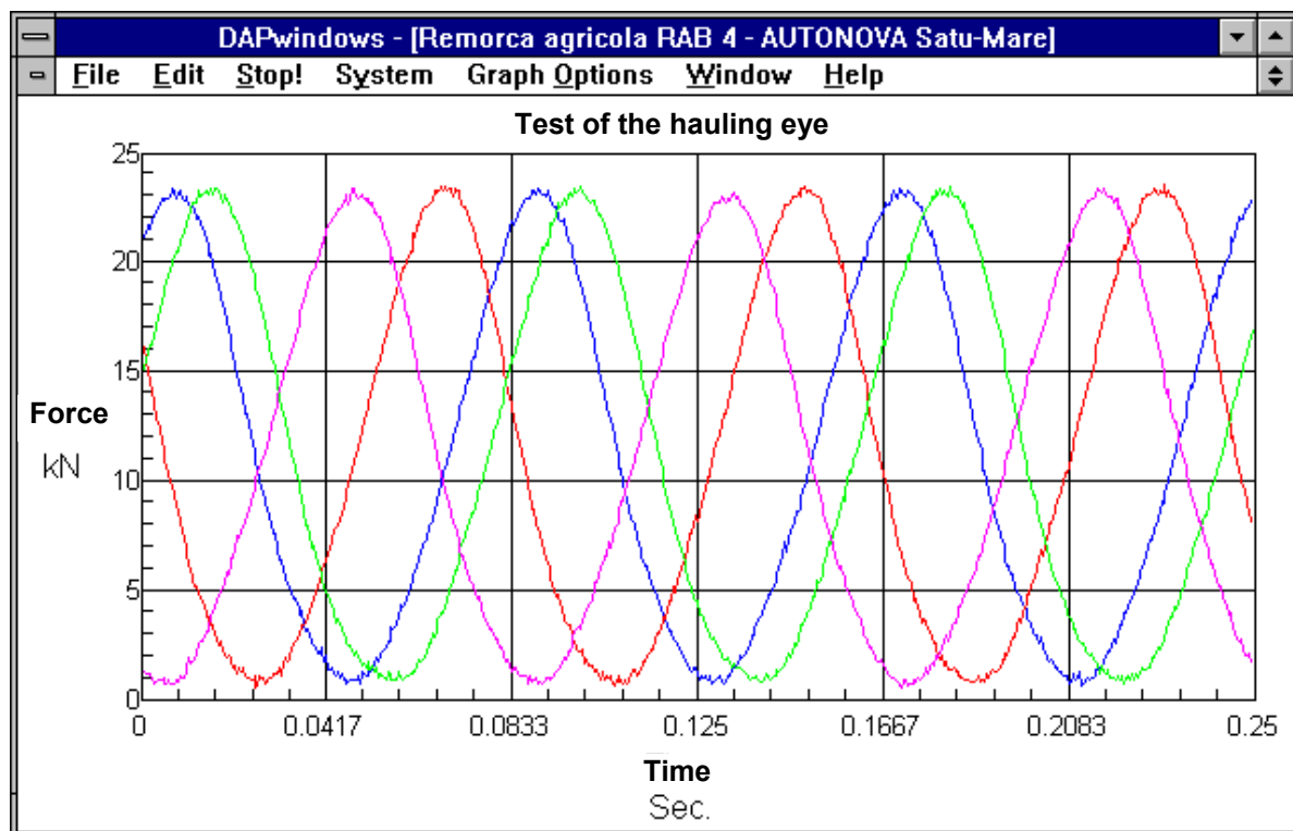
Figure 2 - Force-time diagram for the hauling eye
