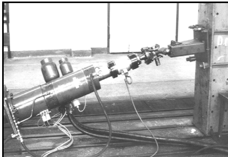
Figure 1 - Assembly performed on the "HYDROPULSE" installation, in order to test the hauling eye
