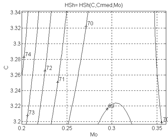
Fig.5. The level curves of distribution HSh = HSh(C, Cr_{med}, Mo)
