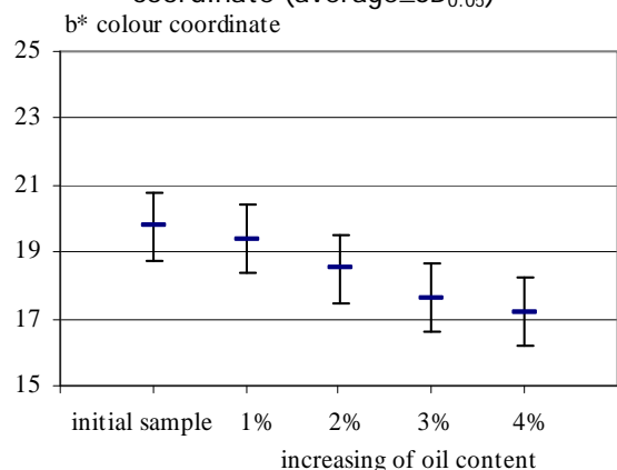
Fig. 3. Result of variance analysis of yellowness coordinate (average \pm SD 0.05 )
