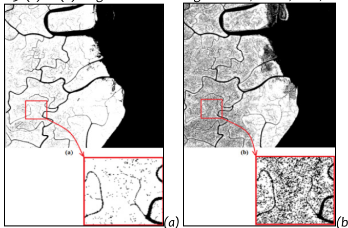
Figure 4. Features detected by LSM from, (a) Multispectral image, (b) Panchromatic image.
