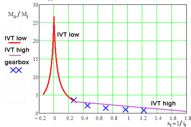
Figure 4. Torque amplification as function of IVT (inverse of) speed ratio
