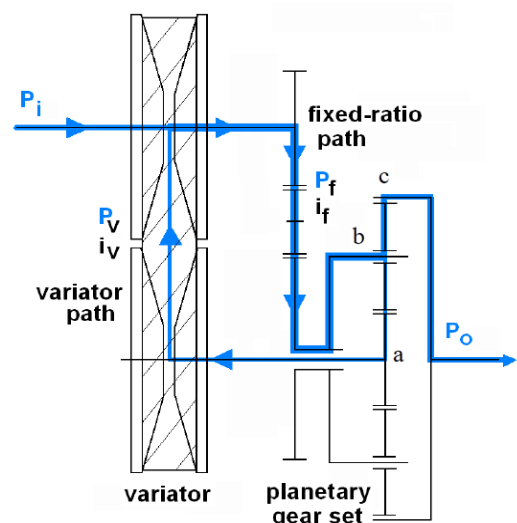
Figure 2. Scheme of a power-split CVT
