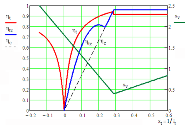
Figure 5. Comparison of the mechanical efficiency for an IVT and a conventional CVT
