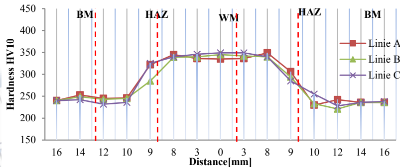
Figure 7. Hardness HV10 - line A, B, C (TOPOCORE 838 B)
