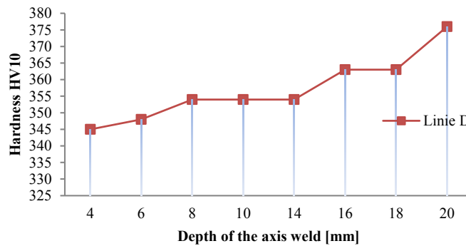
Figure 6. Hardness HV10 in the axis of the weld - line D (Thermanit MTS 616)
