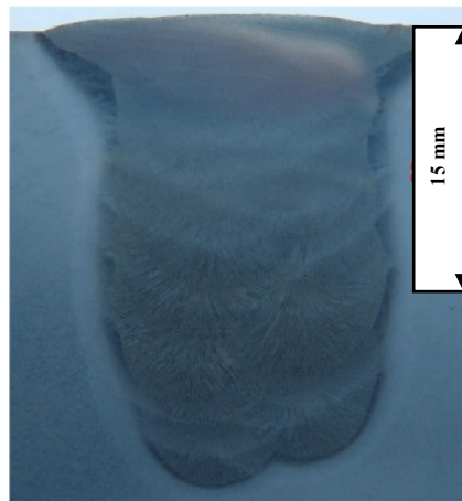
Figure 3. Specimen (PM TOPCORE 838 B)
