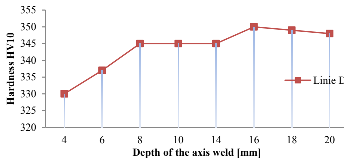
Figure 8. Hardness HV10 in the axis of the weld - line D (TOPOCORE 838 B)
