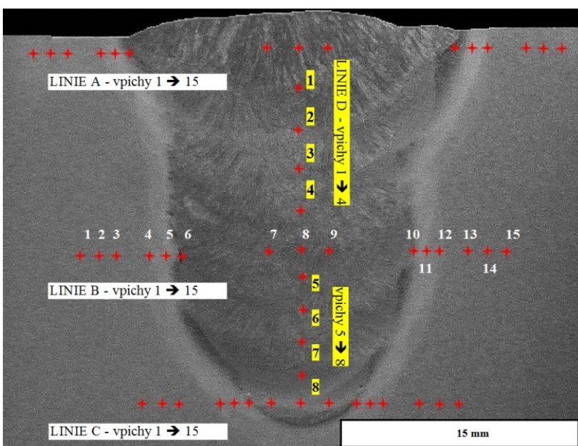
Figure 4. Measurement of hardness HV10 - diagram lines
