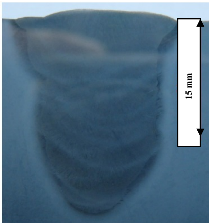
Figure 2. Specimen (PM Thermanit MTS 616)
