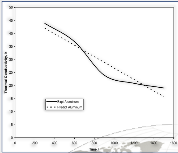
Figure 4: Graphical comparison of experimental and simulated Thermal Conductivity results of Aluminum
