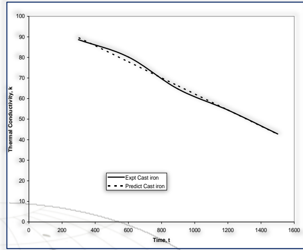
Figure 5: Graphical comparison of experimental and simulated Thermal Conductivity results of Cast Iron
