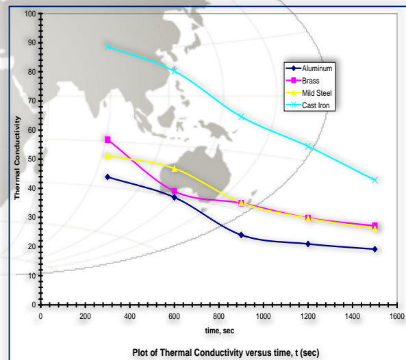
Figure 3: Theoretical results of calculated thermal conductivities
