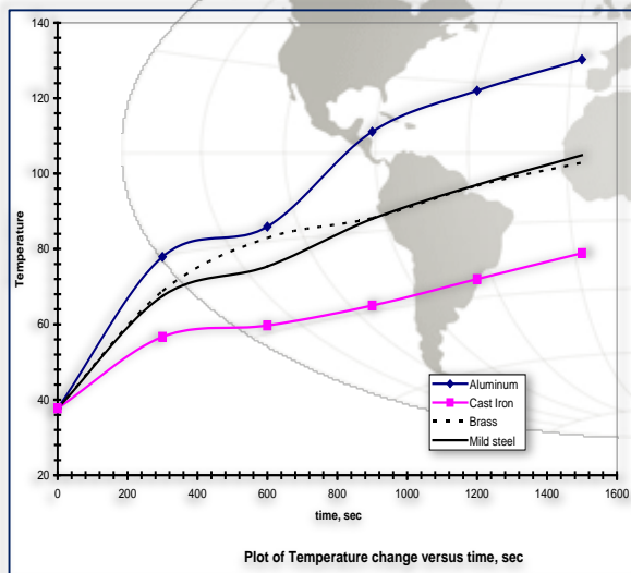
Figure 2: Experimental results of temperature change of each specimen in °C
