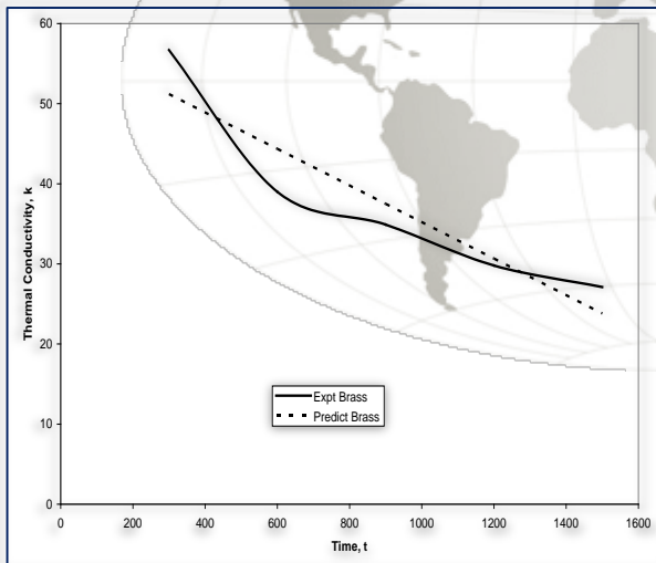
Figure 6: Graphical comparison of experimental and simulated Thermal Conductivity results of Brass
