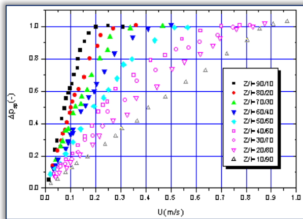
Figure 6. The minimum fluidization velocity mixture of zeolite ( d_p = 0.5 mm) and polyethylene
