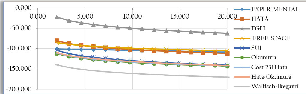
Figure 2: Comparison of measured and simulated received power for Kwara TV.
