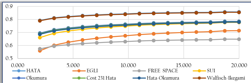
Figure 5: Comparison of Path loss error function value for the eight models
