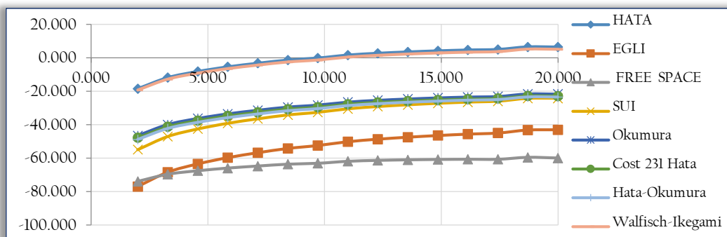
Figure 4: Comparison between mean errors of predicted path loss of eight models
