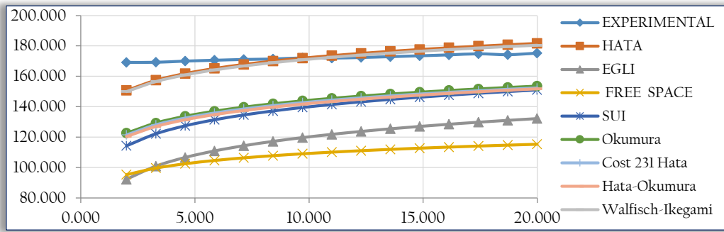
Figure 1: Comparison of measured and simulated path losses for Kwara TV.
