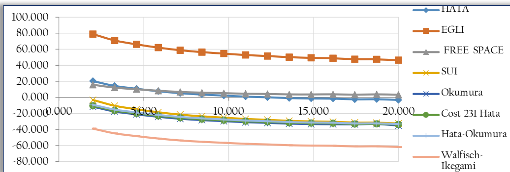
Figure 3: Comparison between MEAN ERROR simulated and measured path losses for NTA, Oshogbo.
