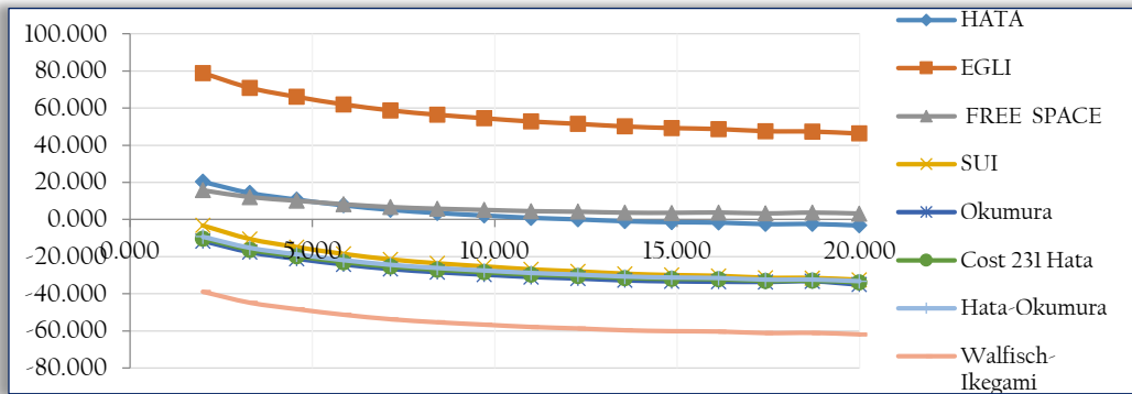
Figure 5: Comparison between mean errors of predicted received power of eight models
