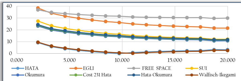
Figure 6: Comparison of Path loss standard error precision value for eight models
