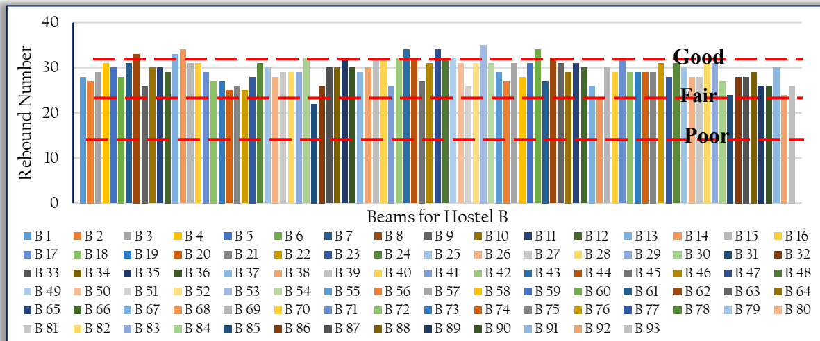
Figure 17: Concrete qualities for Beams of Hostel B
