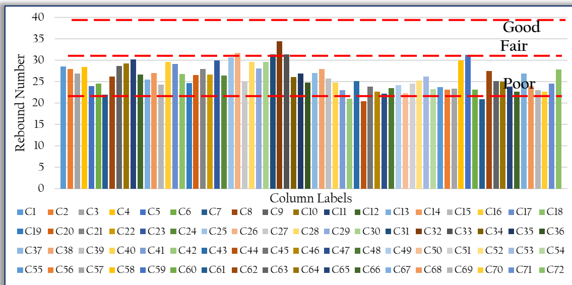
Figure 8: Concrete qualities for ground floor columns for Hostel A
