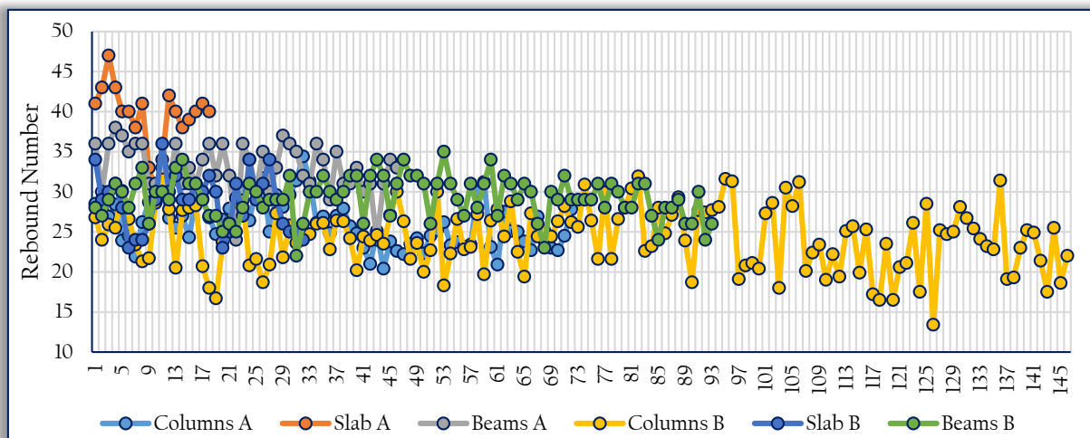
Figure 19: Comparison of Rebound Numbers for Columns, Slab and Beams for Hostel A and B Hostel B
