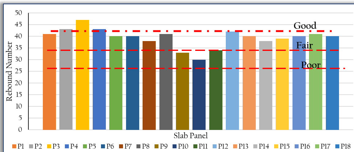
Figure 10: Concrete qualities for Slab of Hostel A
