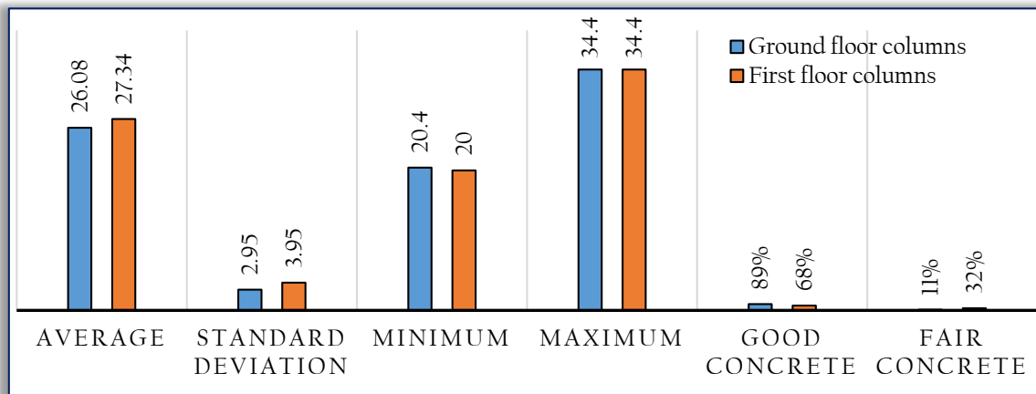
Figure 7: Rebound number plot for ground and first floor columns for Hostel A
