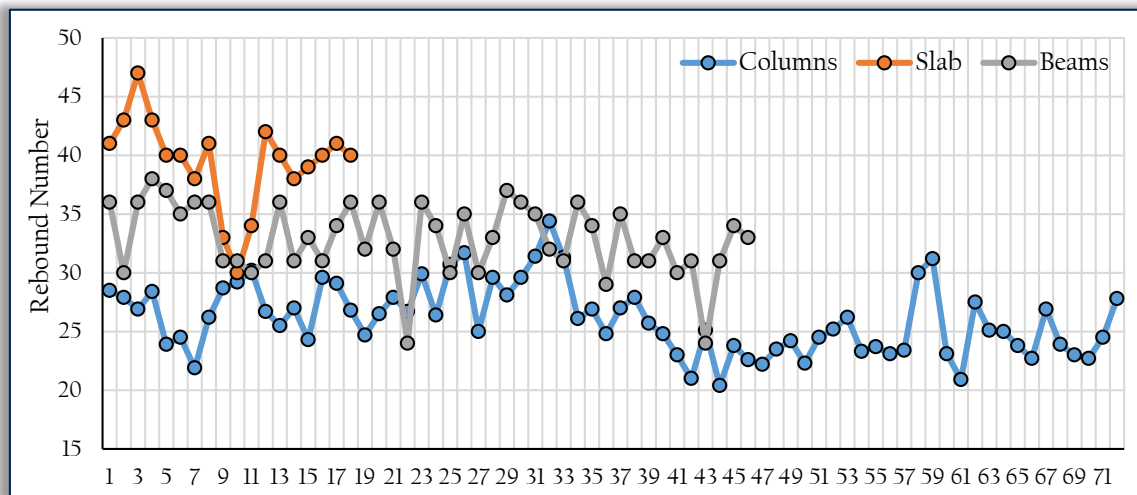
Figure 13: Comparison of Rebound Numbers for Columns, Slab and Beams of Hostel A
