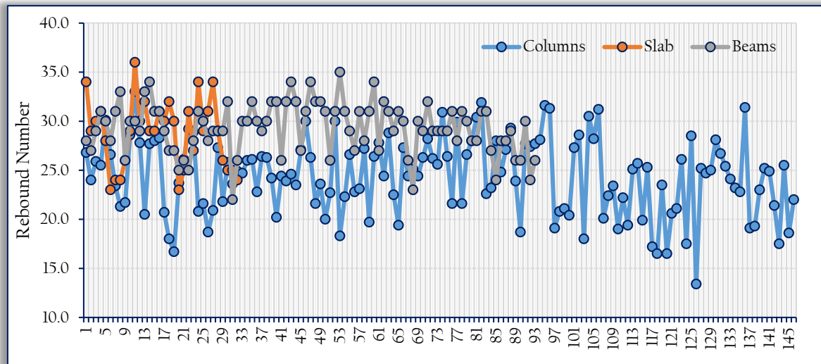
Figure 18: Comparison of Rebound Numbers for Columns, Slab and Beams for Hostel B
