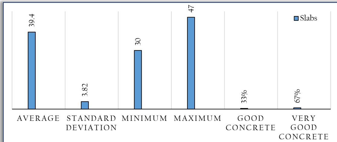
Figure 9: Rebound number plot for slabs of Hostel A
