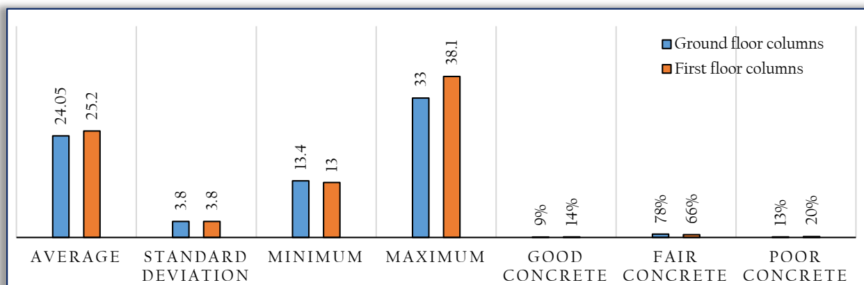
Figure 14: Rebound number plot for ground and first floor columns for Hostel B
