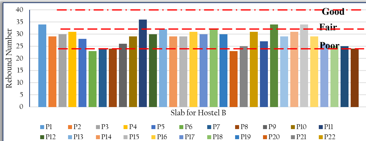
Figure 16: Concrete qualities for Slab of Hostel B
