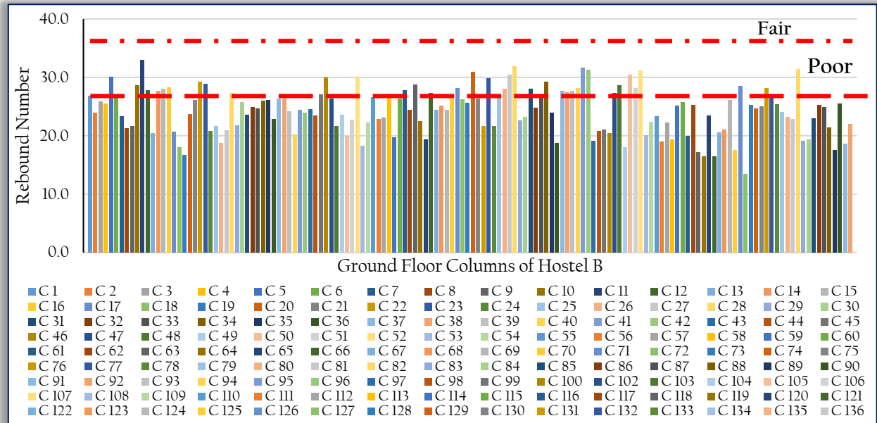
Figure 15: Concrete qualities for ground floor columns of Hostel B
