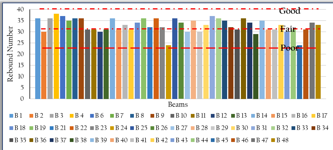
Figure 12: Concrete qualities for first floor beam labels of Hostel A
