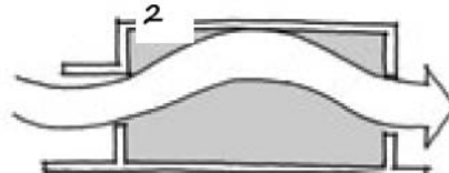
Figure 3e. 1. Providing a slot between a canopy or 'eye-brow' can increase downward pressure and result in a more comfortable air flow within a room. 2. Solid overhangs, or 'eye-brows', directly over a window can direct airflow upward away from the occupied zone of a room
