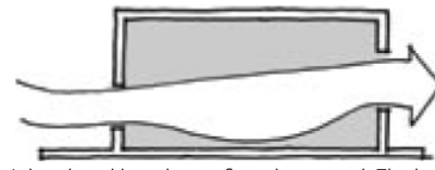
Figure 3d. Inlet placed low directs flow downward. The location of the outlet has no effect on the internal flow pattern
