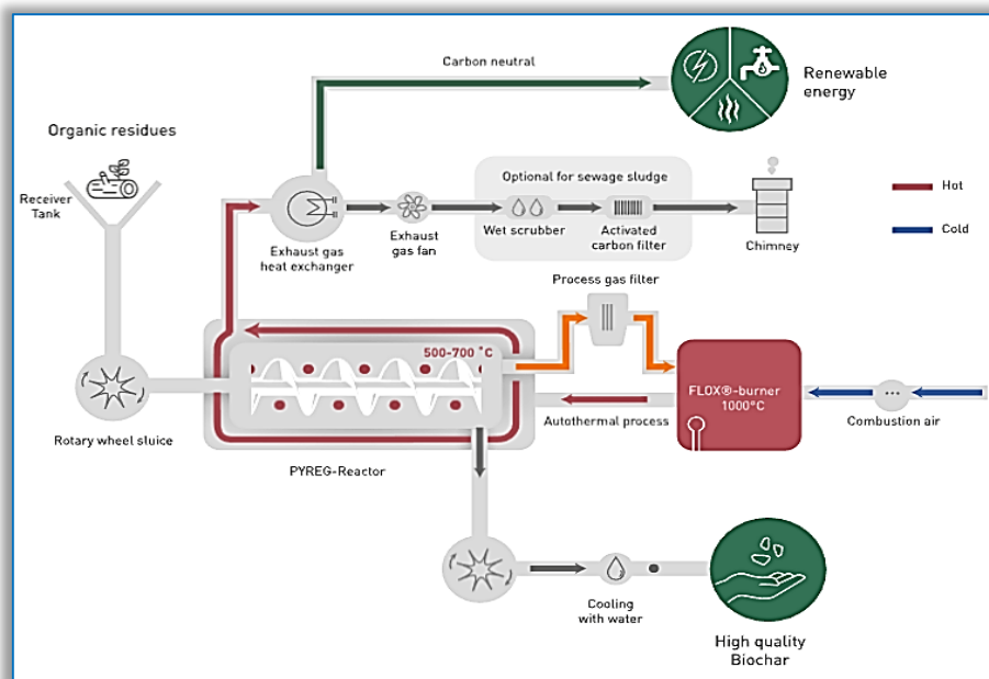
Figure 4 – The technological process of an installation (Pyreg processes ( https://pyreg.com/our-technology/ ))
