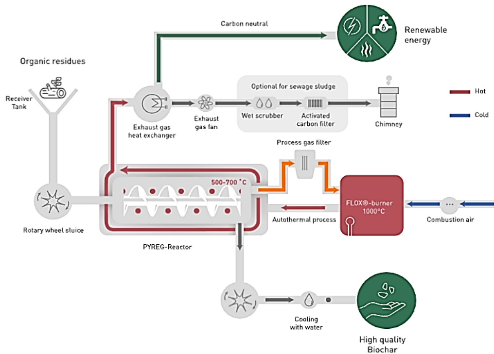
Figure 4 – The technological process of an installation (Pyreg processes ( https://pyreg.com/our-technology/ ))
